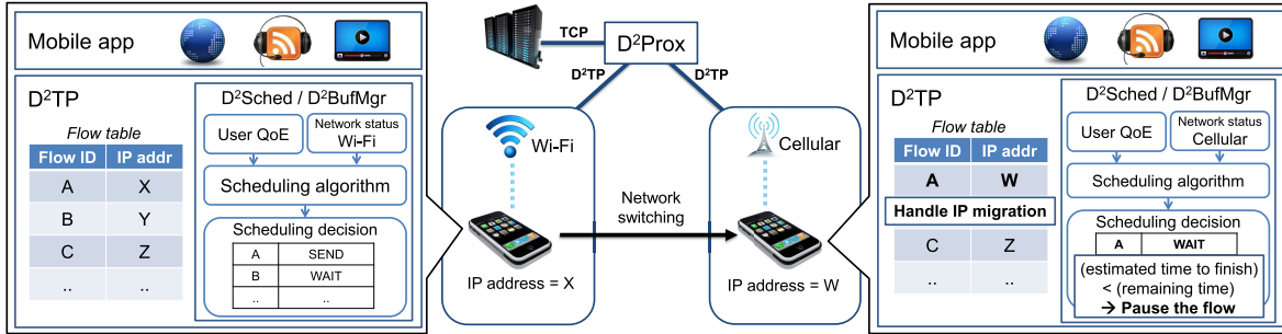
Fig. 1. Cedus delayed data offloading architecture. D 2 TP handles both network disruptions and long delays. D 2 Sched schedules the flows for delayed Wi-Fi offloading (e.g., it uses a Wi-Fi connection as much as possible but sometimes switches to an LTE network to finish in time).
