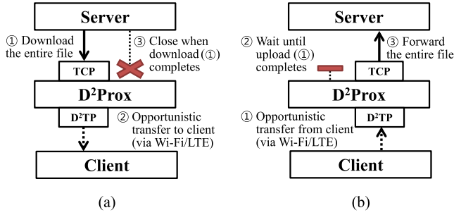
Fig. 4. Protocol translation in D²Prox. (a) D²Prox on download case. (b) D²Prox on upload case.
